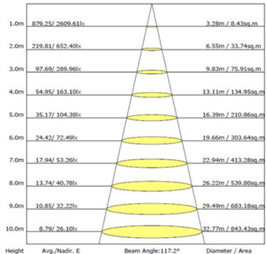
Illuminance at a Distance
