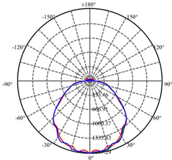
Light Distribution Curve [Unit:cd]
