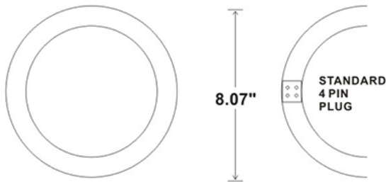
STANDARD 8" CIRCLELINE LAMP
