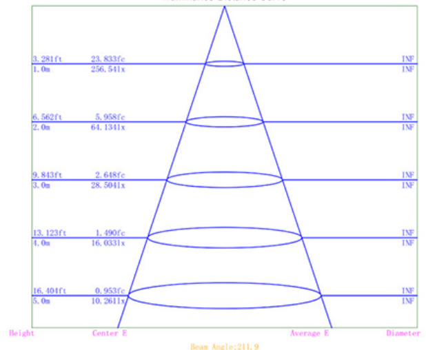
Illuminance-Distance Curve
