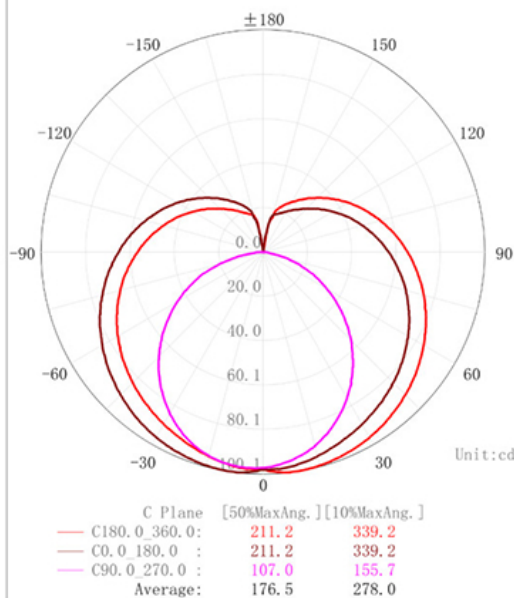
C Plane Distribution Diagram
