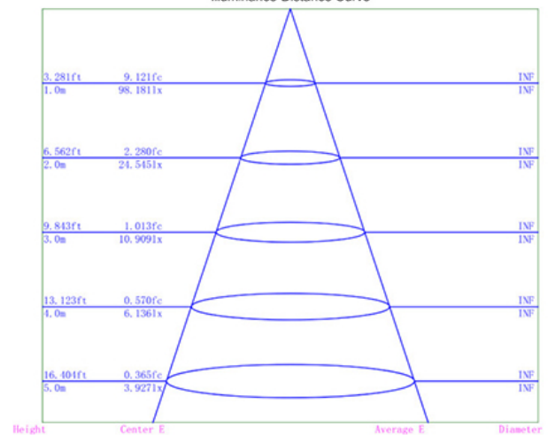
Illuminance-Distance Curve
